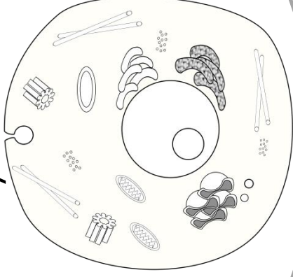
Eukaryotic Cell
