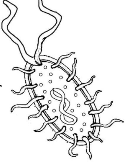
Prokaryotic Cell
